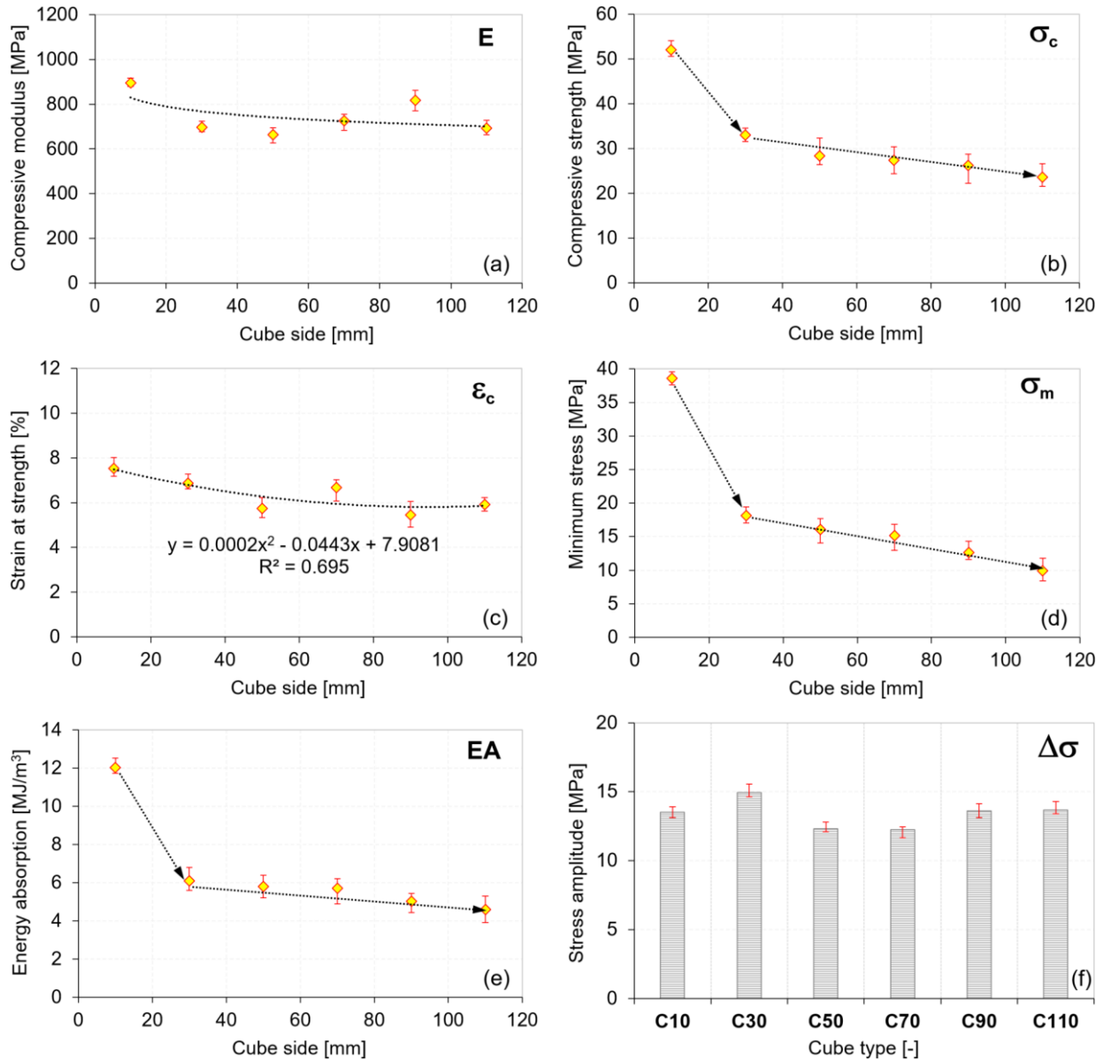
Fig. 5 – Main properties of the FFF-printed PLA parts.
