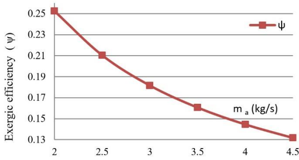
Fig. 2 – Exergy efficiency change of the amount of air passing through the condenser surface.
