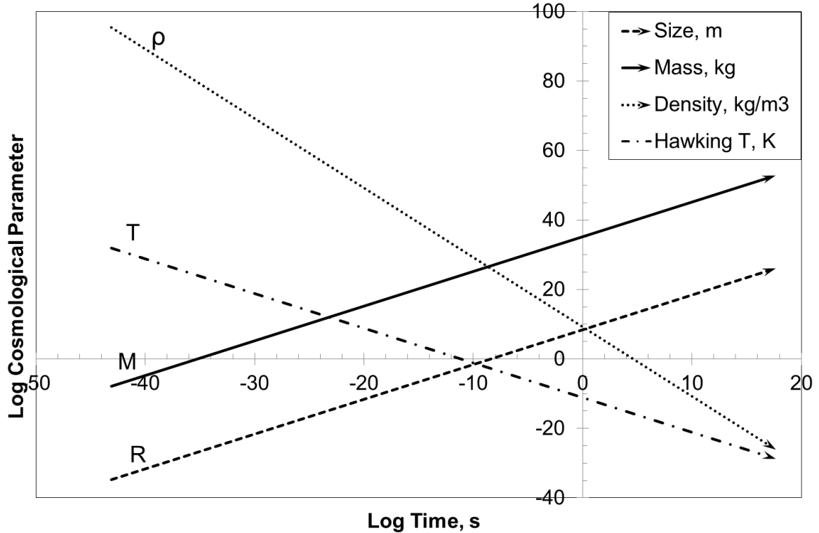
Fig. 1 – Time course of cosmological parameters during the expansion.
