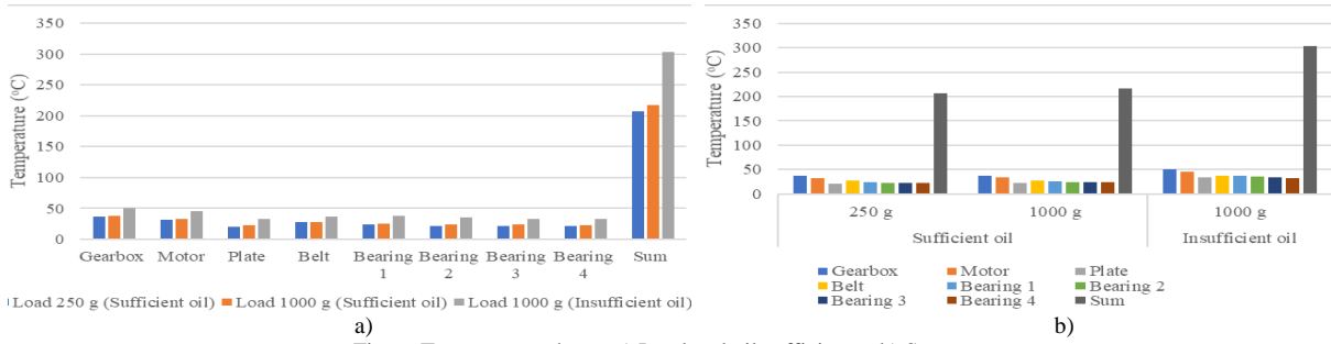
Fig. 6 Temperature charts; a) Load and oil sufficiency, b) Setup components
