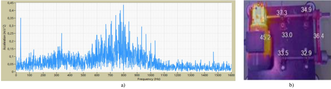
Fig. 4 a) Spectrum domain for condition of insufficient oil with 1000 g load, b) Thermal inspection for condition of insufficient oil with 1000 g load
