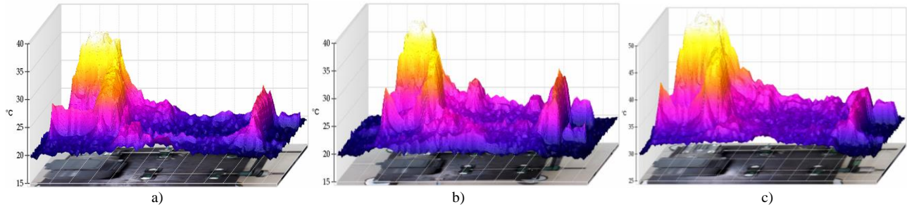
Fig. 7 Infrared thermal distributions; a) 250 g load under condition of sufficient oil, b) 1000 g load under condition of sufficient oil, c) 1000 g load under condition of insufficient oil
