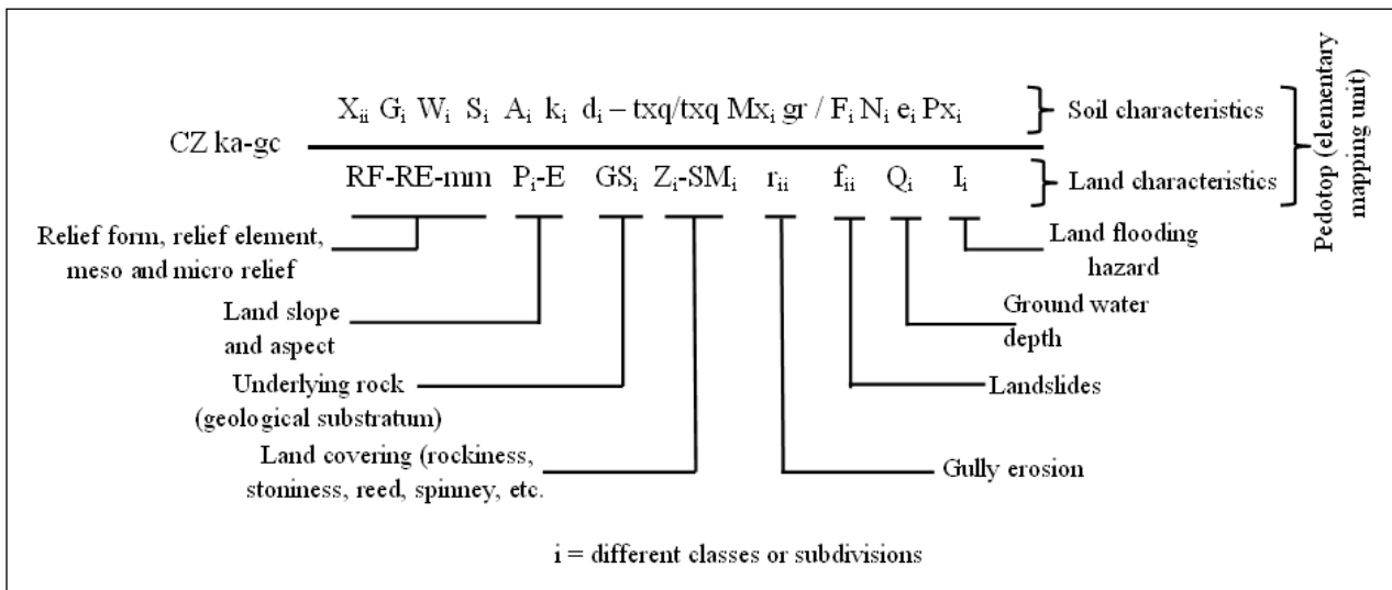
Figure 2. Formula of elementary soil - land unit used in soil survey in Romania for maps at large scales (see Figure 1 for explanations of the numerator symbols)
